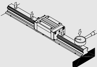
Final tightening of mounting bolts
