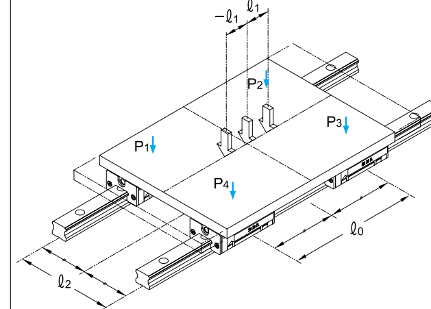
Condition 5 Horizontal axis with rail movable
