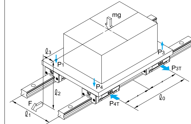
Condition 8 Horizontal axis with inertia
