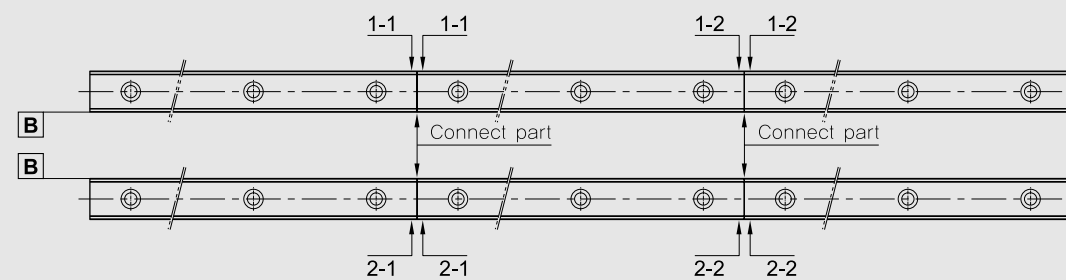
2 axis application and multiple rail joining method
