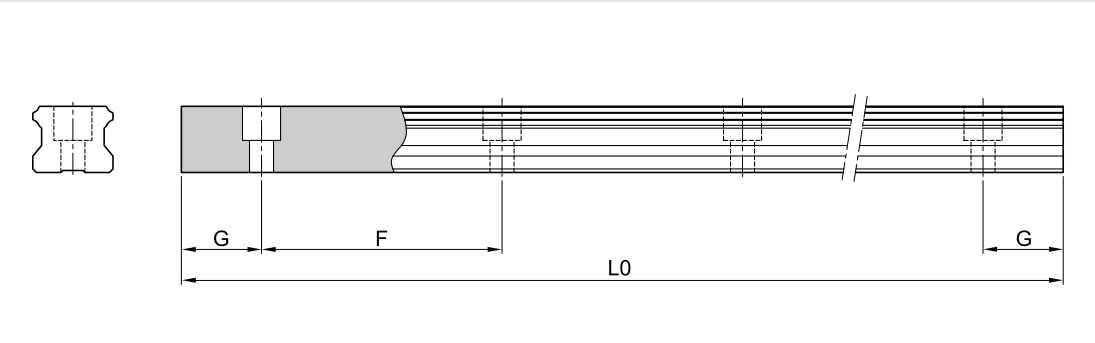
Standard and Max. Length of SBI rail
