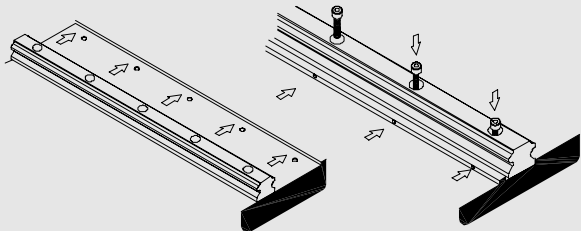
Final tightening of mounting bolts
